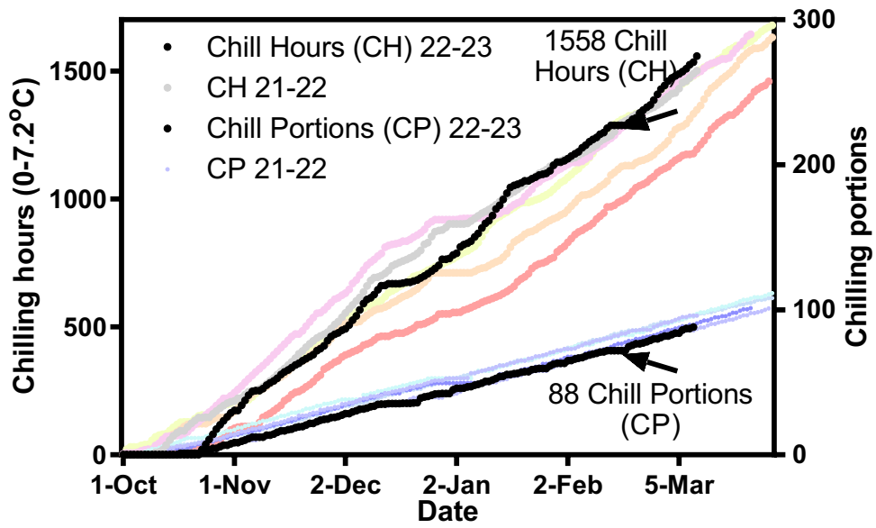
Figure 5. Seasonal accumulation of chilling hours (0-7.2 °C) and dynamic chill portions starting on October 1, 2022.
