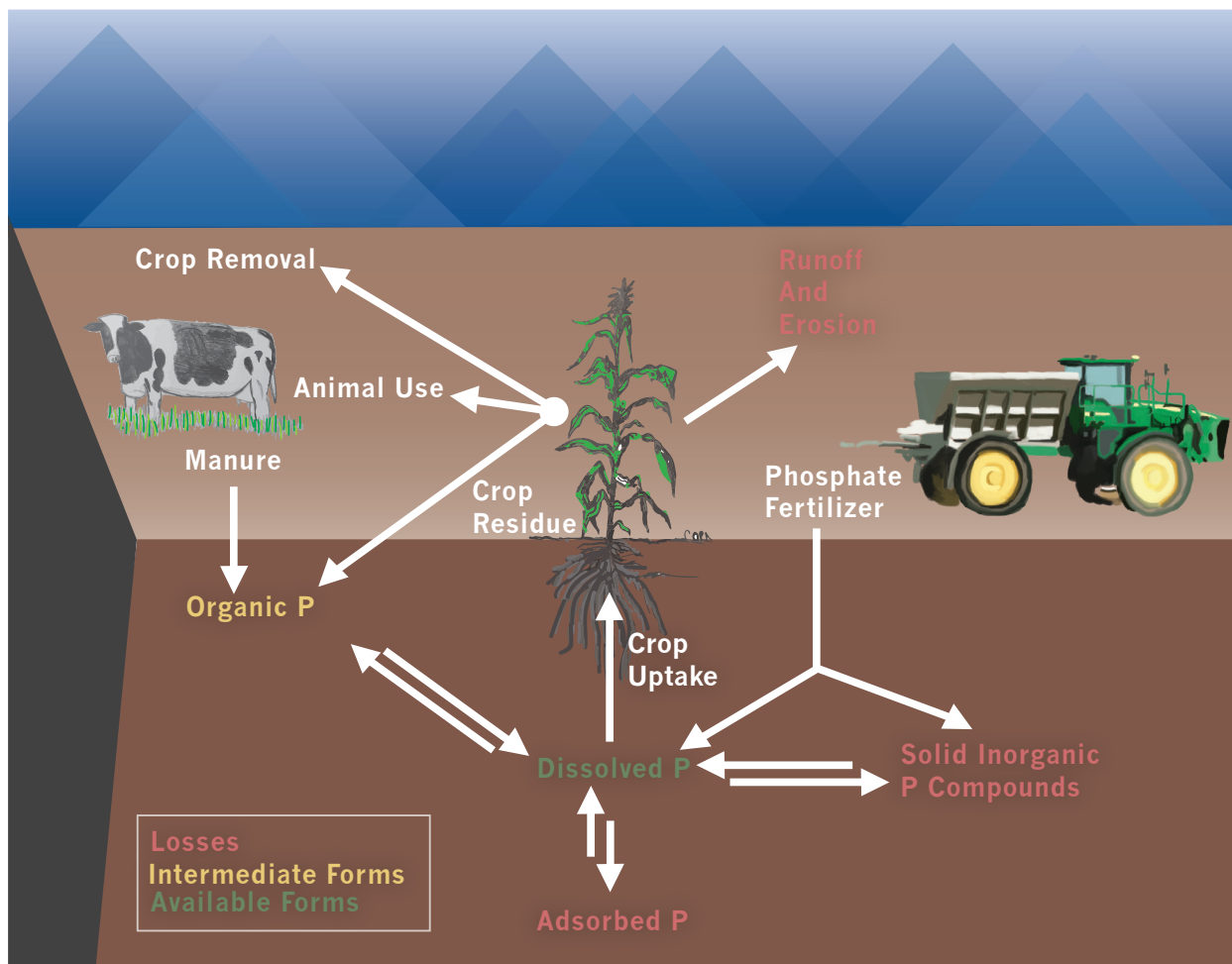
Figure 1. The phosphorus cycle in agricultural soils.
